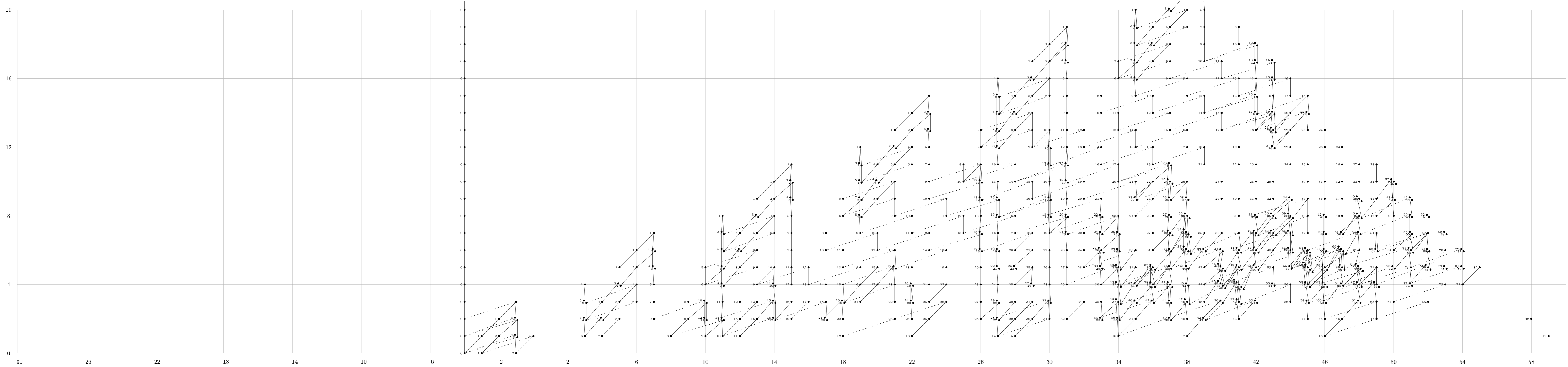
Figure 4: P_{-4} , -30 \leq n \leq 60 , 0 \leq s \leq 20
